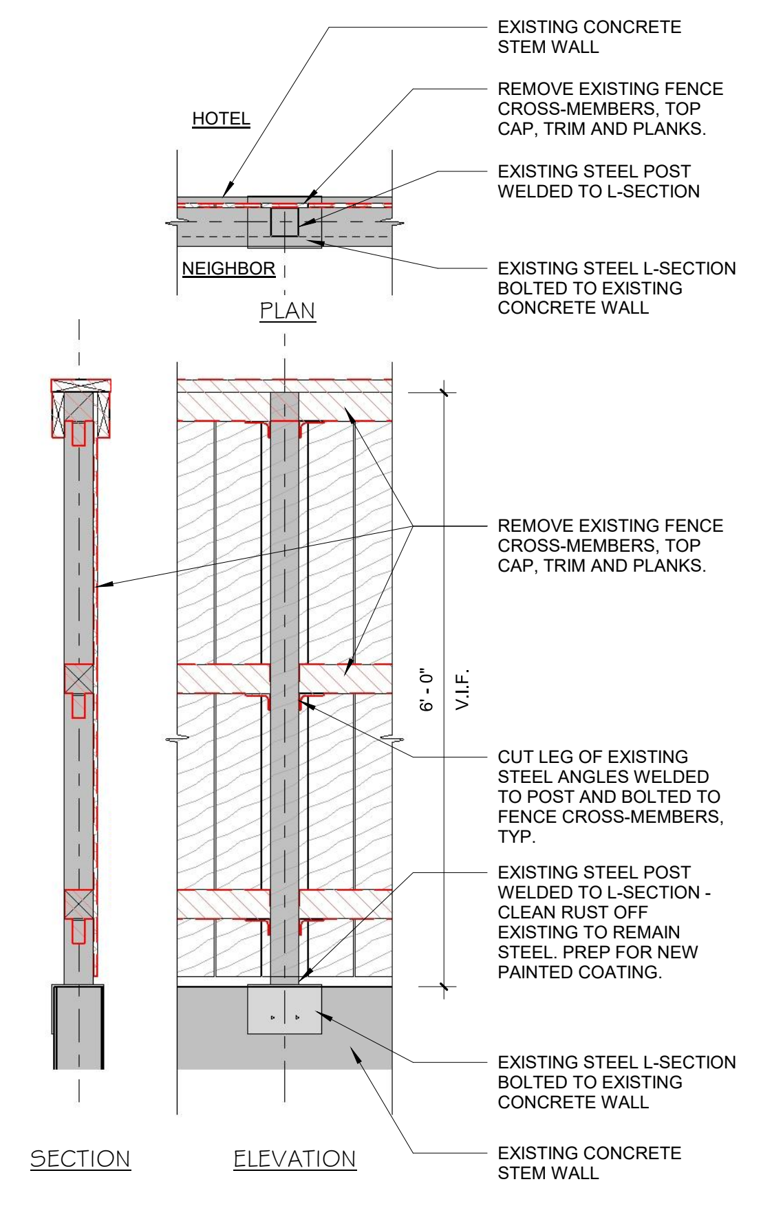
4 FENCE DETAIL - DEMO 3/4" = 1'-0"
