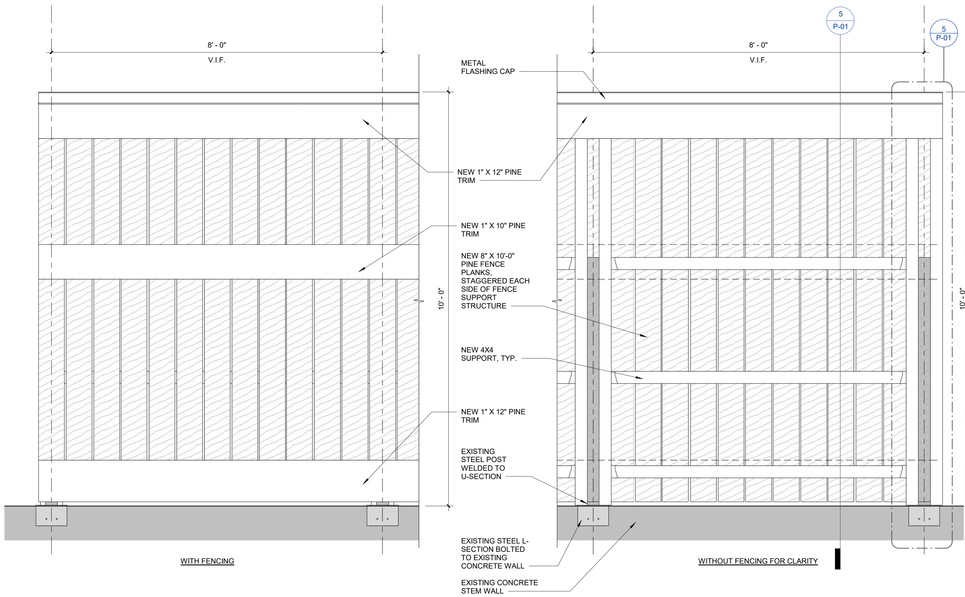
7 FENCE ENLARGED ELEVATION 3/4" = 1'-0"
