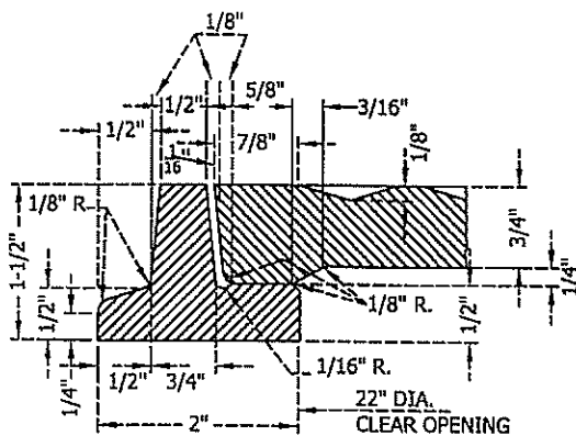
CROSS SECTION THRU RIM
