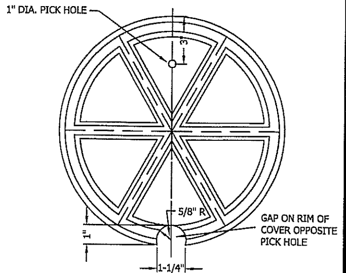
BOTTOM OF MANHOLE COVER
