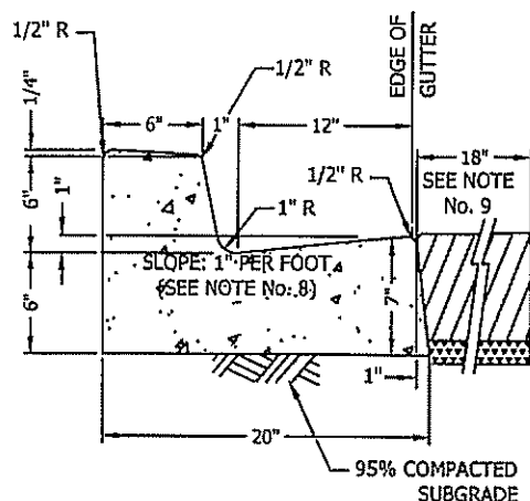
STANDARD 6" CURB AND 12" GUTTER
