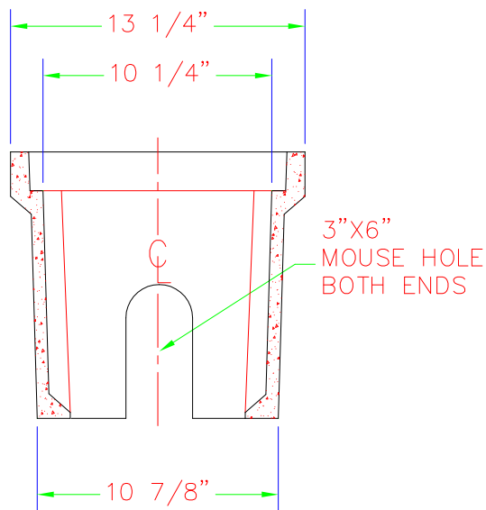
SECTION B-B
