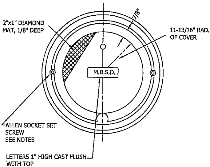
TOP OF MANHOLE FRAME & COVER
