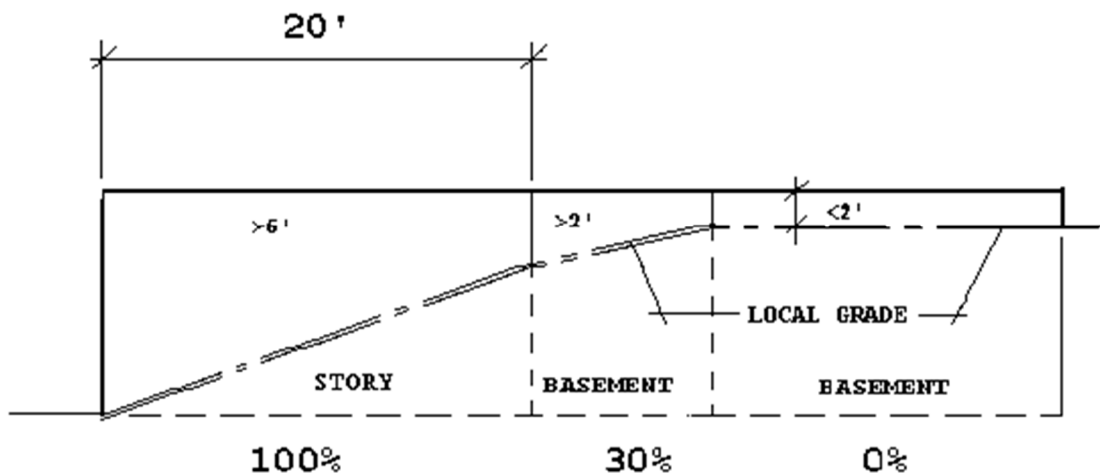
PROPOSED BASEMENT/STORY CONDITIONS COUNTED AS BFA
