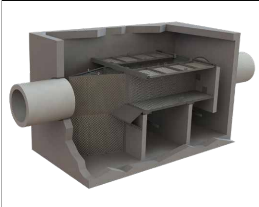
Debris Separating Baffle Box
