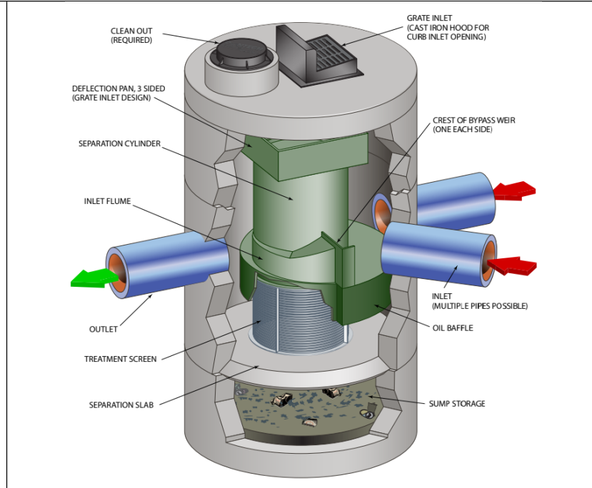
Hydrodynamic Separator
