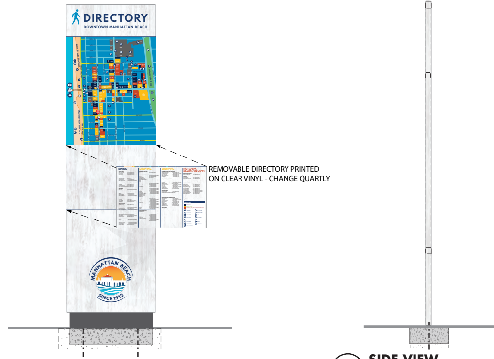
2 REMOVABLE DIRECTORY scale: 1/2" = 1' -0"
