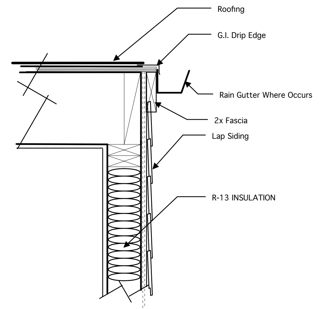
Rake Detail 4-A5
