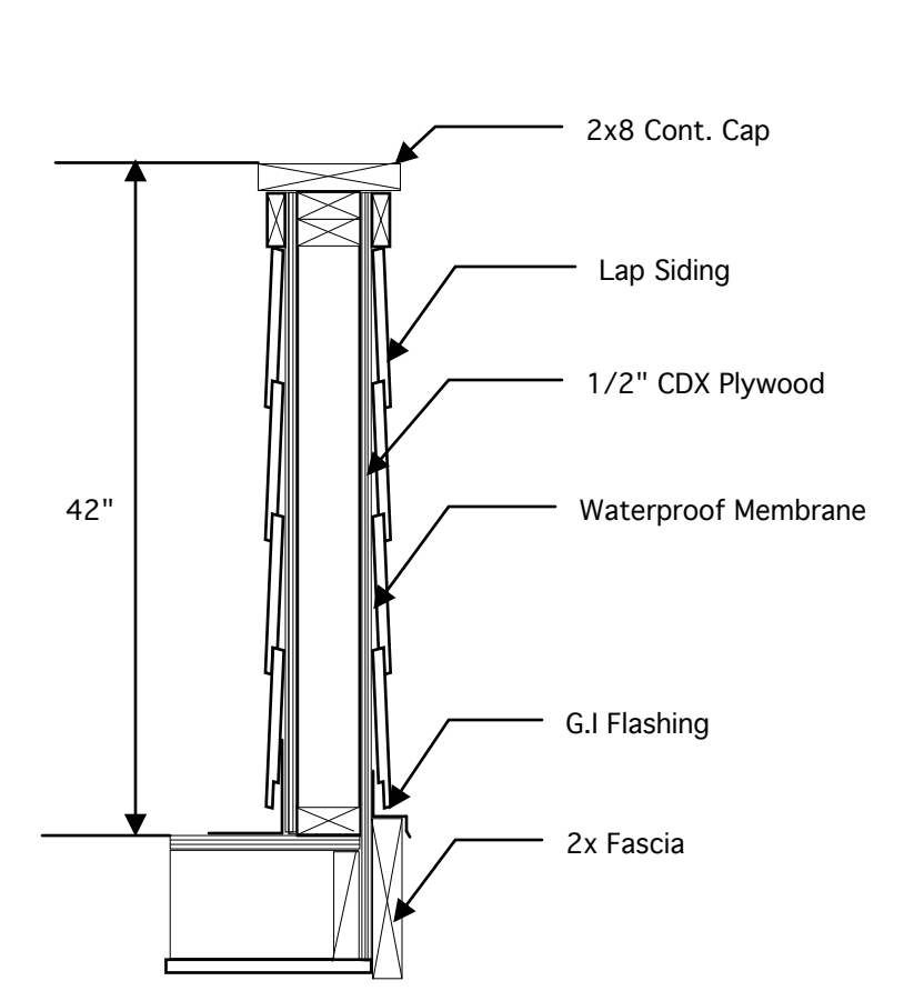
Exterior GuardRail Wall Detail 3-A5
