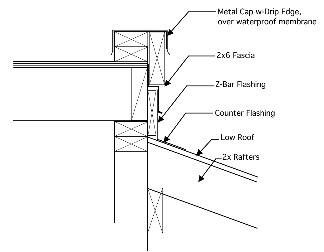
Wall To Low Roof Detail 2-A5
