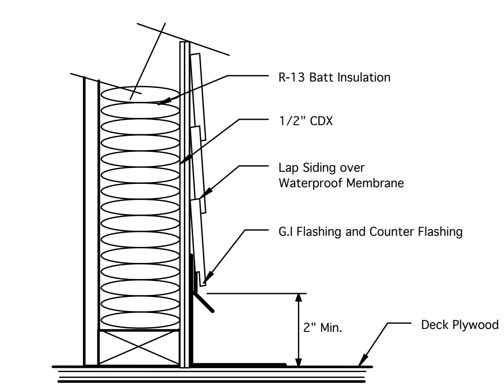
Wall Base At Deck 1-A5
