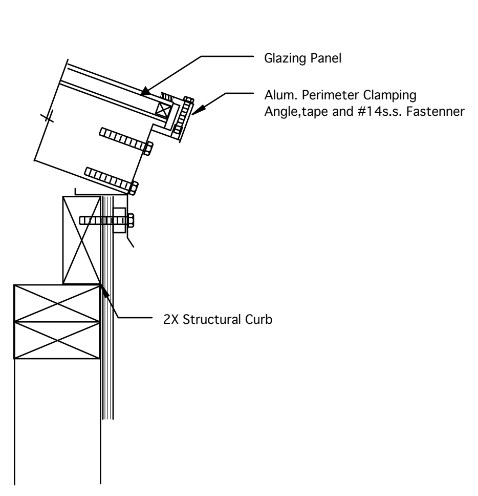
Skylight Curb Detail 5-A5
