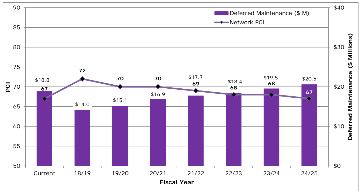
Figure 10: PCI vs. Deferred Maintenance for Scenario 2
