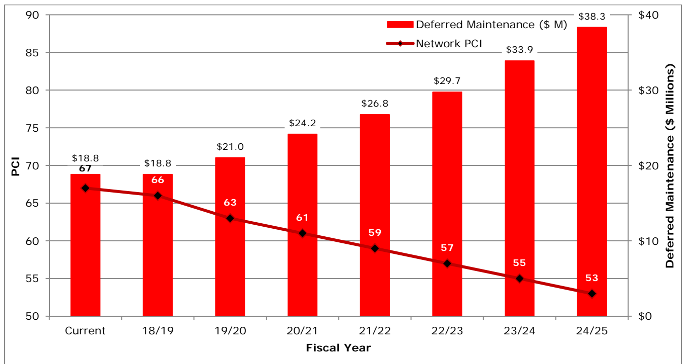
Figure 13: PCI vs. Deferred Maintenance for Scenario 5
