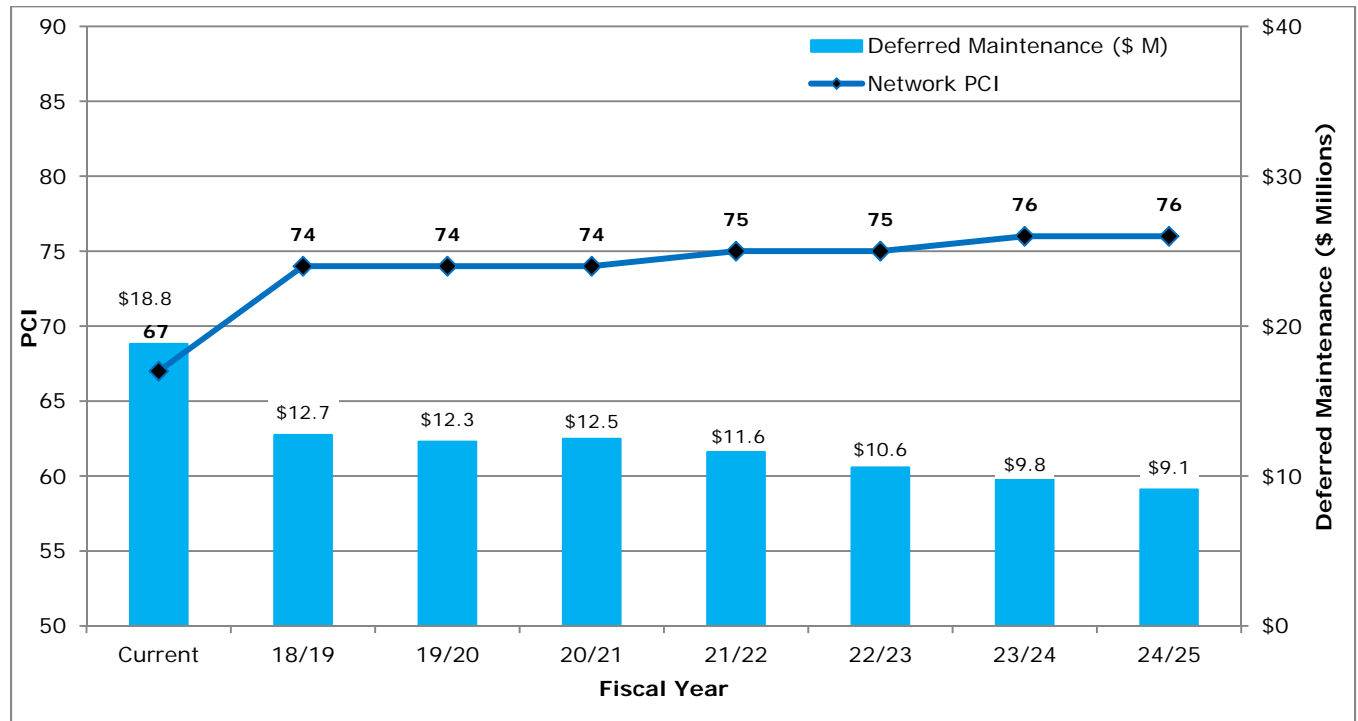
Figure 11: PCI vs. Deferred Maintenance for Scenario 3
