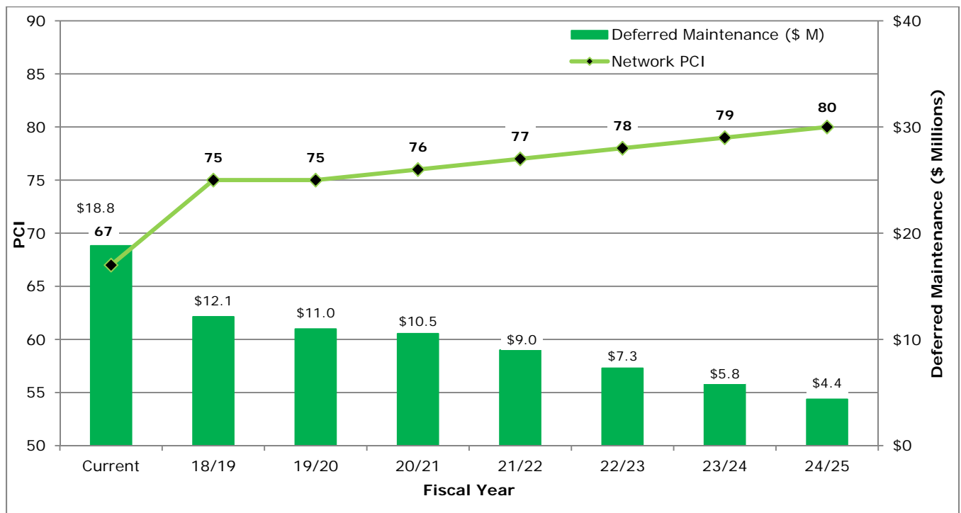
Figure 12: PCI vs. Deferred Maintenance for Scenario 4
