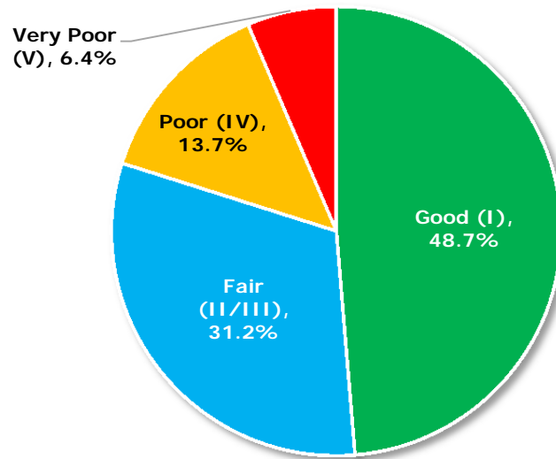
Figure 6: Pavement Network Breakdown by Condition Category
