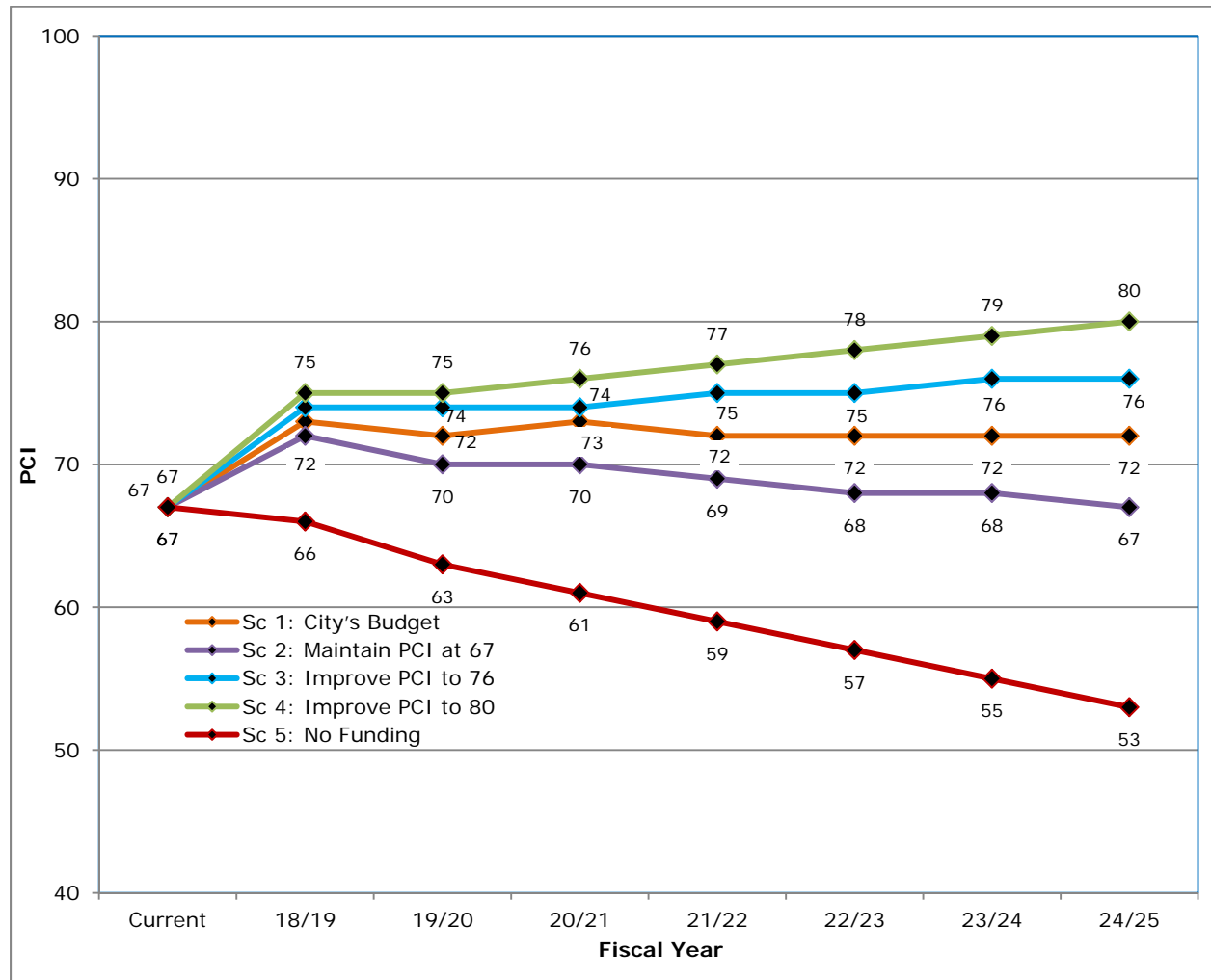
Figure 14: PCI Comparisons between Scenarios
