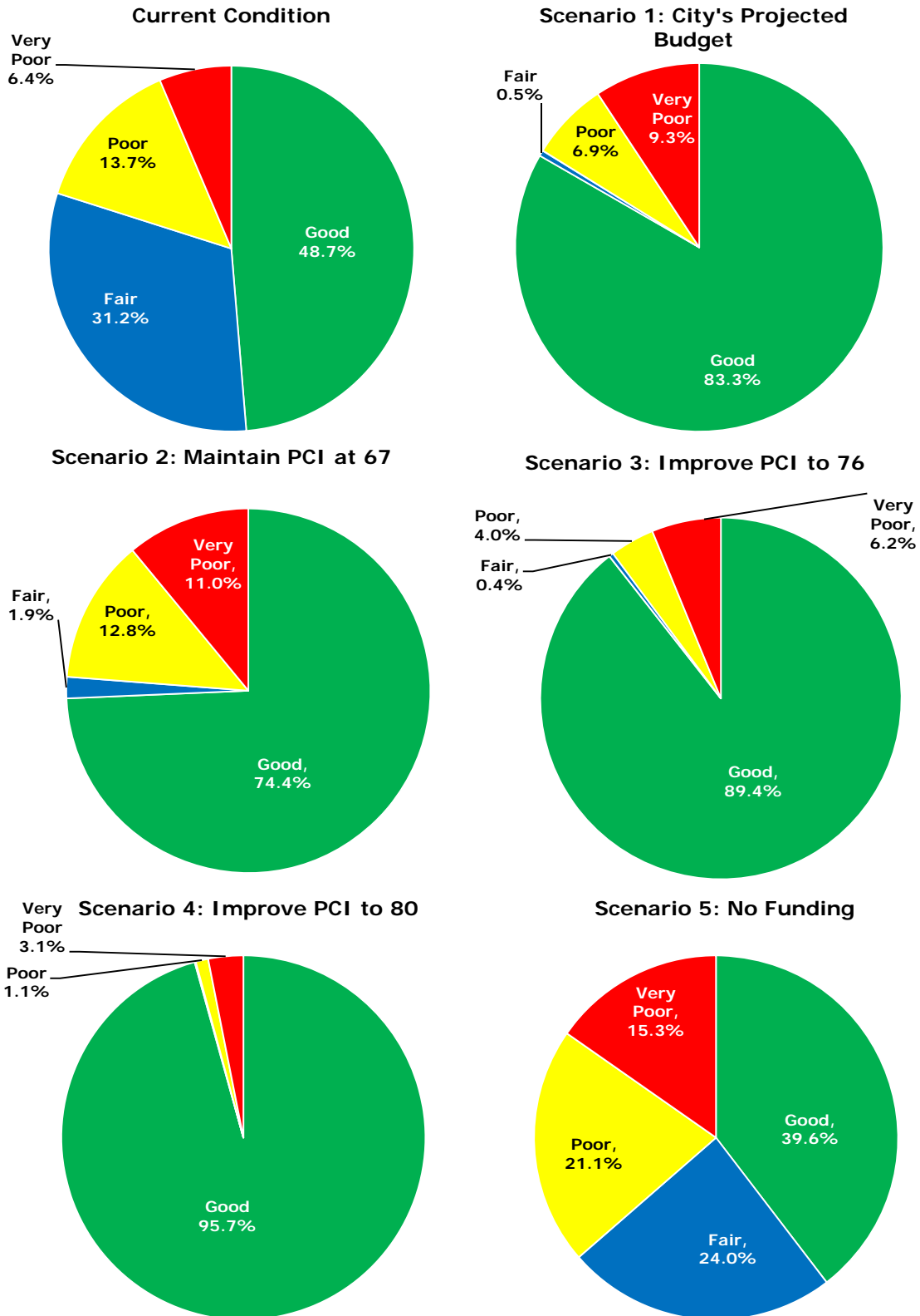
Figure 16: Resulting Pavement Network Condition Breakdown for Budget Scenarios
