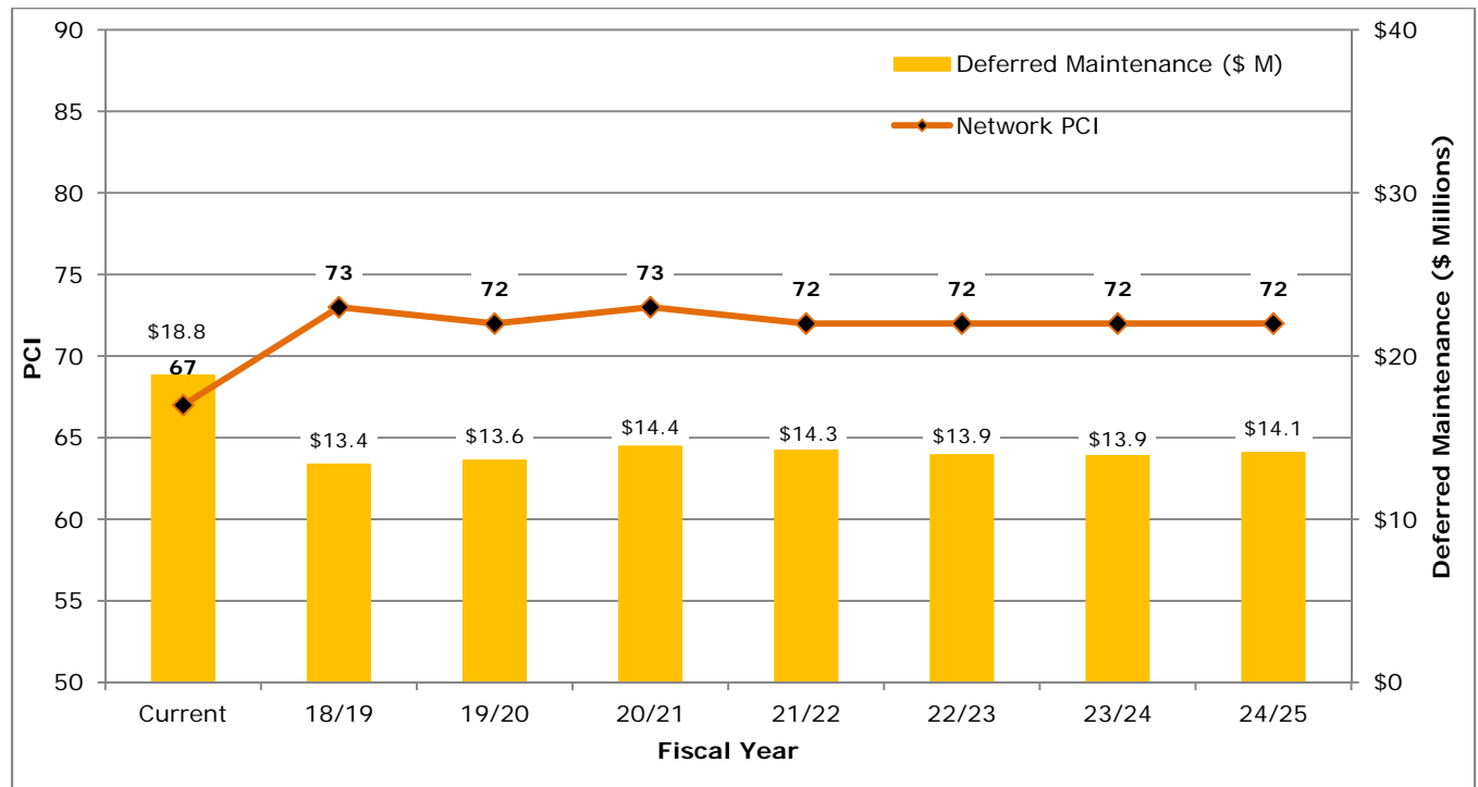
Figure 9: PCI vs. Deferred Maintenance for Scenario 1
