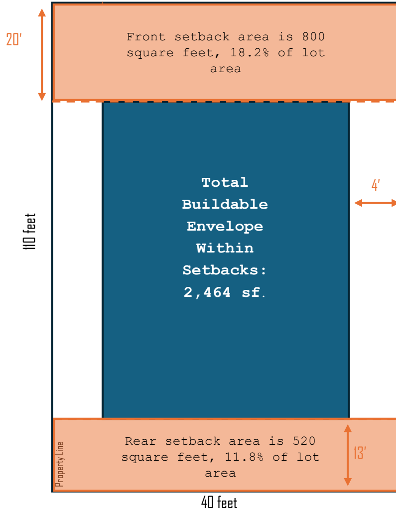
Example 1 Typical 40' x 110' Lot Setbacks
