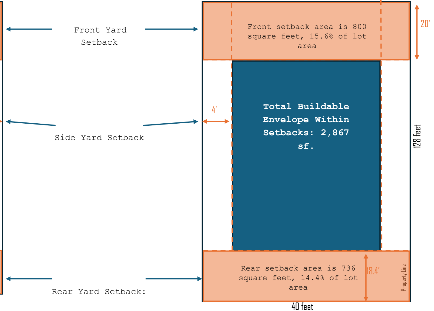
Example 2 Typical 40' x 128' Lot Setbacks
