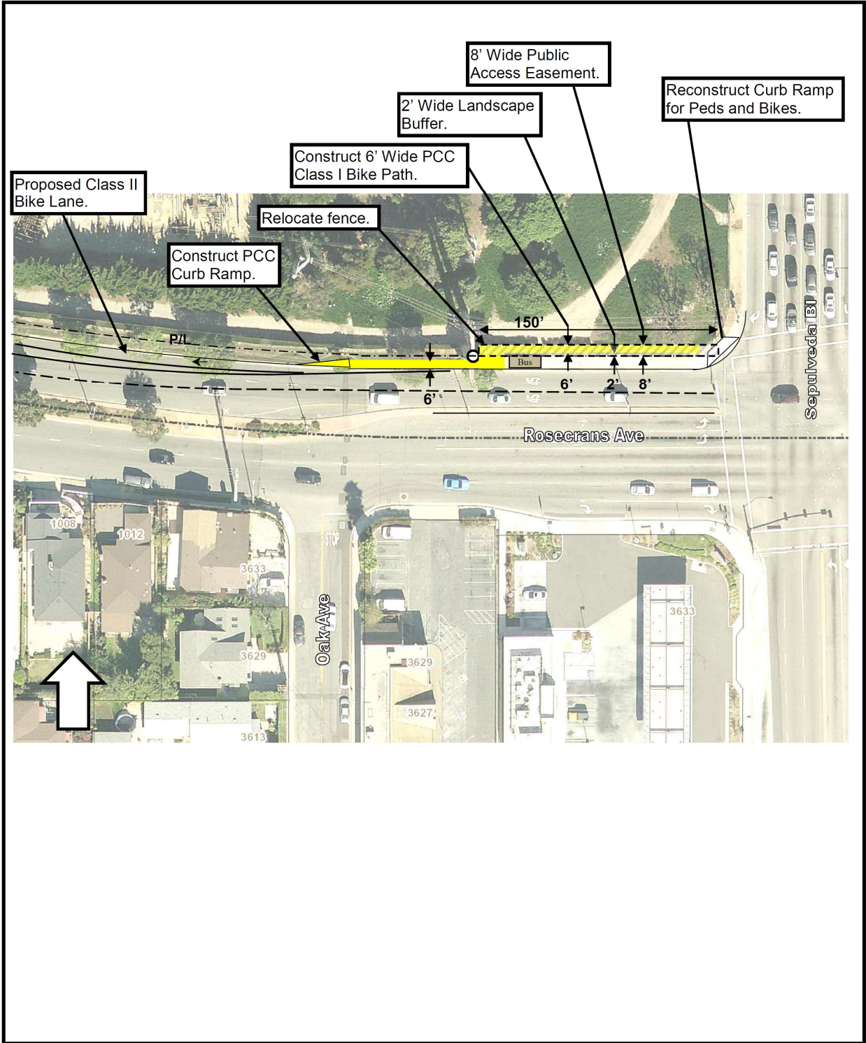
Rosecrans Avenue West of Sepulveda Boulevard Bike Lane Concept Sketch
